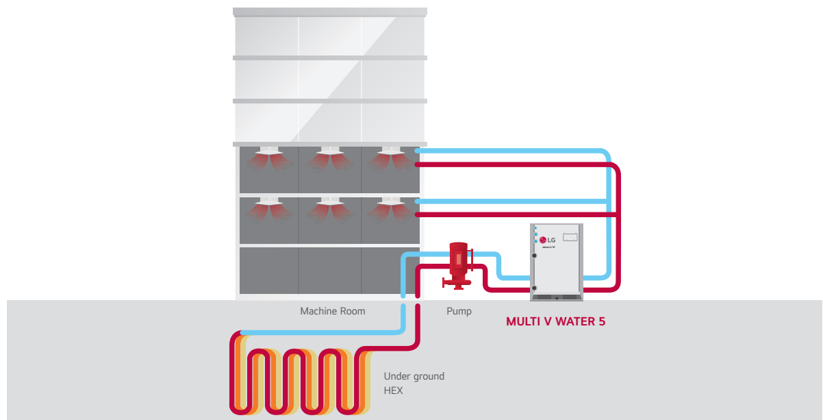
CHILLER - FCU
